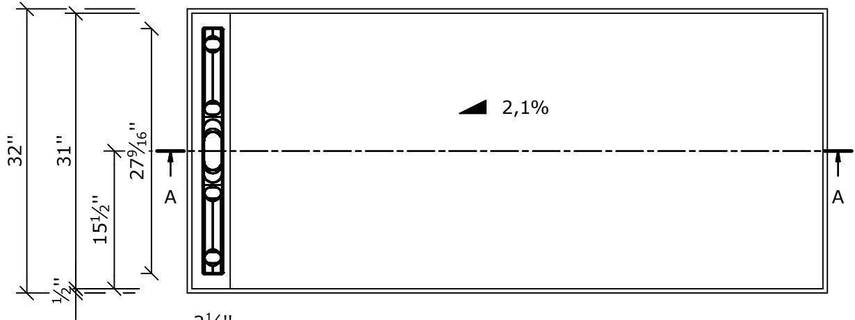
top view (1 : 15)
