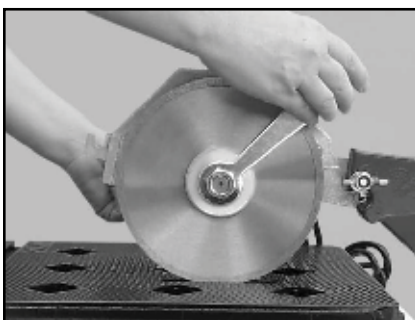
(G) Install the Retaining Nut and Outer Flange, place the Shaft Wrench and Blade Wrench as shown in Step C and Tighten the Retaining Nut
