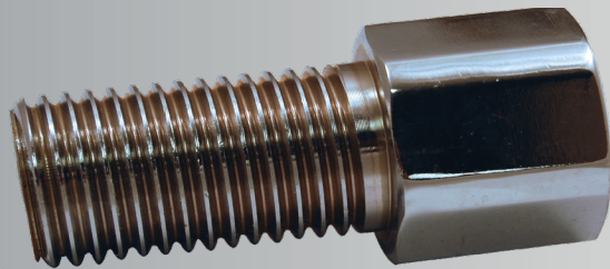
5/8-11 Thread to 1-1/4-7 Thread P/N: 150764
