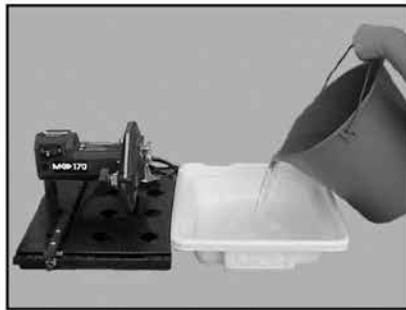
(D) Fill the Water Pan with clean water (this should be done periodically during cutting).
