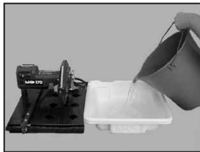
(E) Fill the Water Pan with clean water. Place Cutting Table on Water Pan.
