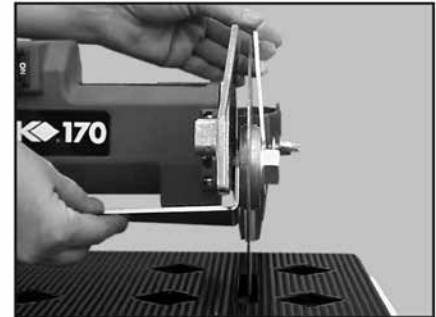
(C) Open the Blade Guard and place the Shaft Wrench on the Motor Shaft and the Blade Wrench on the Blade Retaining Nut.
