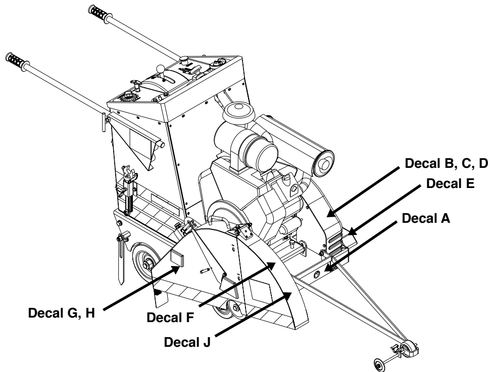
Fig. 2 Norton Clipper Self Propelled Flat Saw Safety Decal Locations
