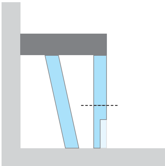
1-cut Discreto Montage The front element can be modified for integration of the Fundo Riolito Discreto wall drain
